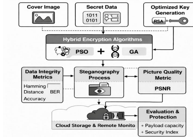
Fig. 2. The IOT-Based Hybrid Image Security Framework
